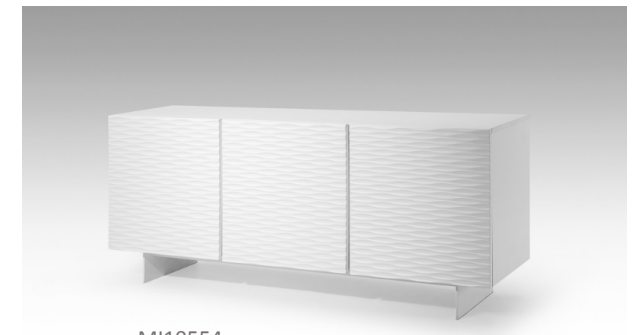
MI10554
